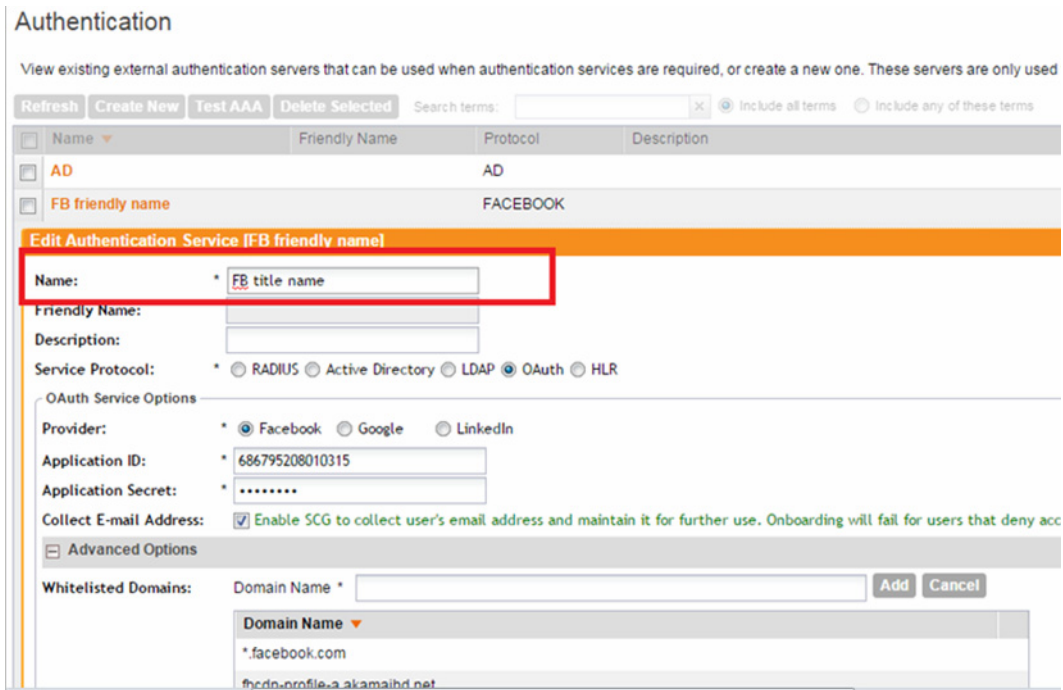
Figure 19. OAuth Provider Configuration
