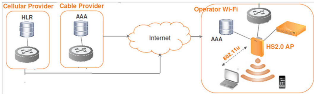
Figure 1. Working of Hotspot 2.0
