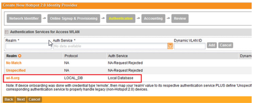
Figure 8. Hotspot Identity Provider - Authentication
